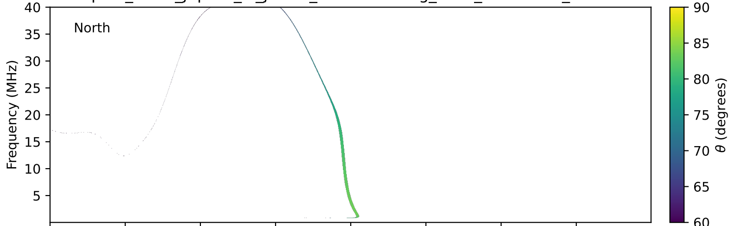
expres_earth_jupiter_io_jrm33_lossc-wid1deg_3kev_20010108_v11.cdf
