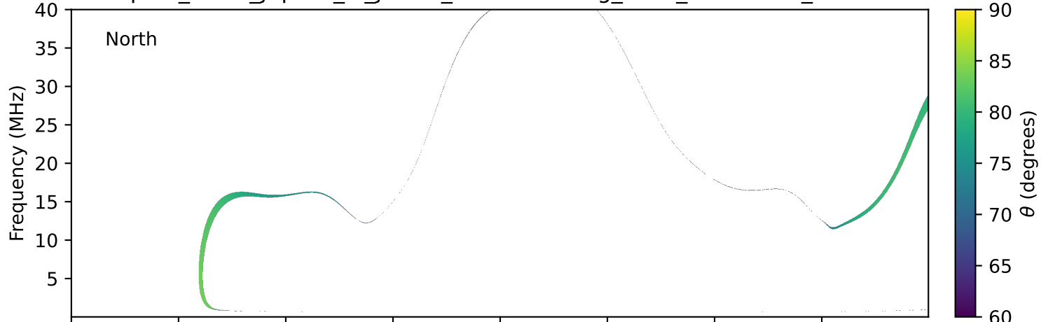
expres_earth_jupiter_io_jrm33_lossc-wid1deg_3kev_20010104_v11.cdf
