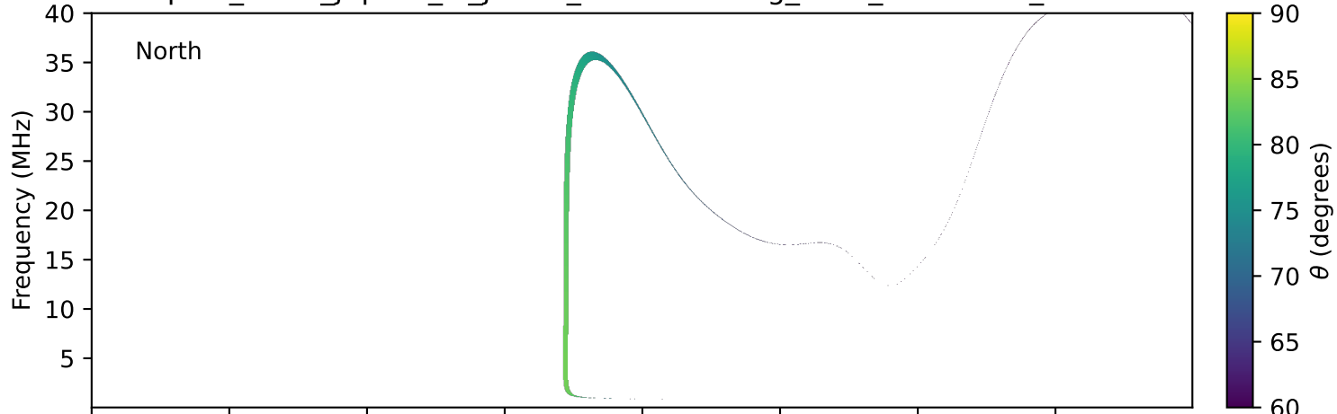
expres_earth_jupiter_io_jrm33_lossc-wid1deg_3kev_20010102_v11.cdf
