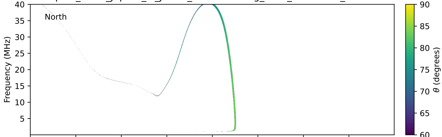
expres_earth_jupiter_io_jrm09_lossc-wid1deg_3kev_20010131_v11.cdf
