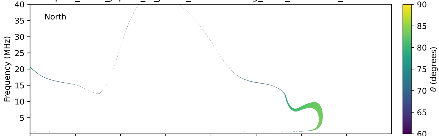
expres_earth_jupiter_io_jrm09_lossc-wid1deg_3kev_20010129_v11.cdf
