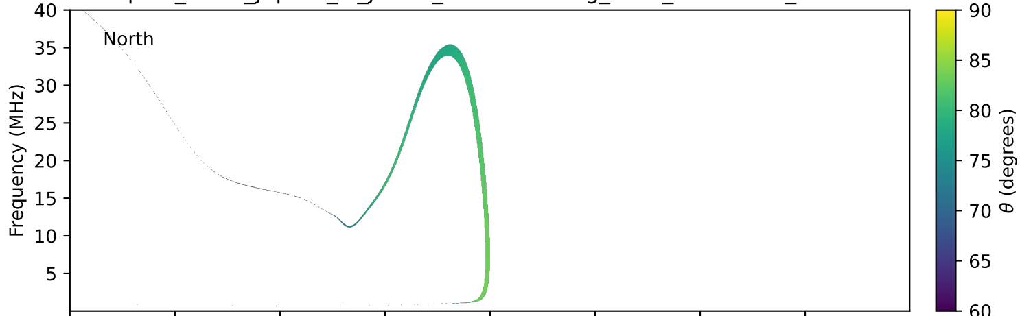
expres_earth_jupiter_io_jrm09_lossc-wid1deg_3kev_20010124_v11.cdf
