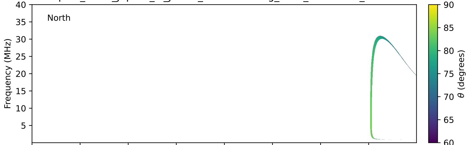
expres_earth_jupiter_io_jrm09_lossc-wid1deg_3kev_20010121_v11.cdf
