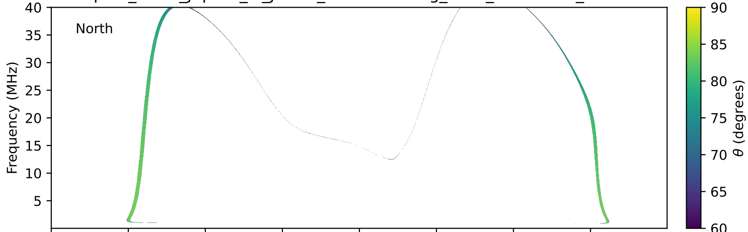
expres_earth_jupiter_io_jrm09_lossc-wid1deg_3kev_20010120_v11.cdf
