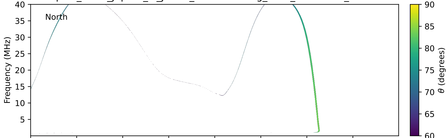
expres_earth_jupiter_io_jrm09_lossc-wid1deg_3kev_20010106_v11.cdf
