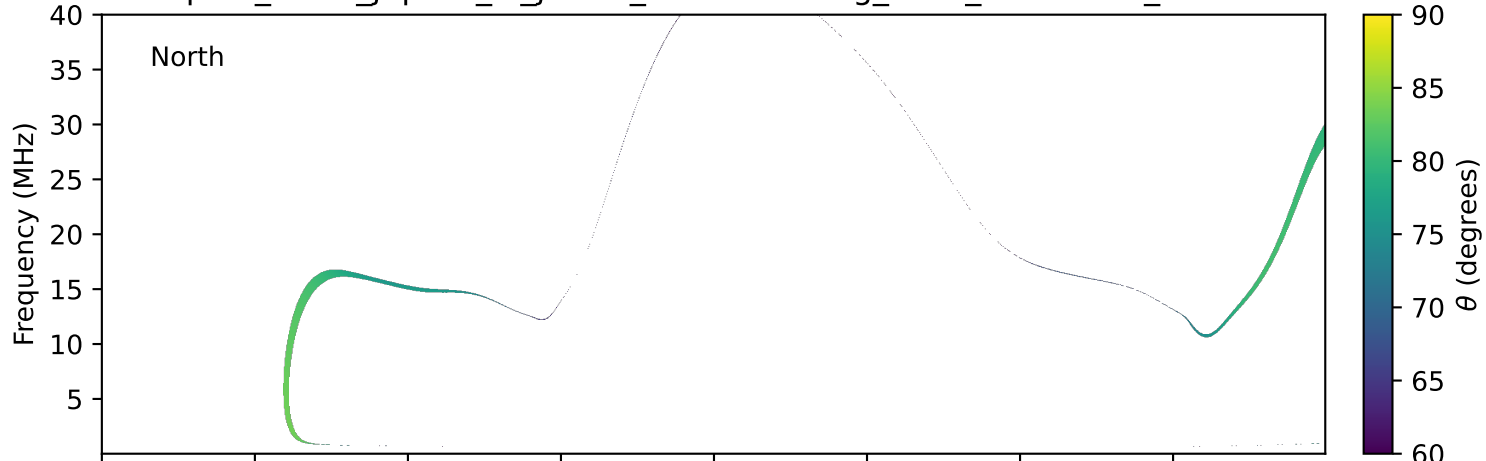
expres_earth_jupiter_io_jrm09_lossc-wid1deg_3kev_20010104_v11.cdf
