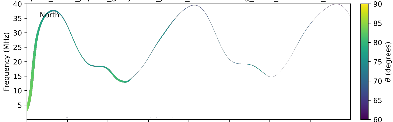
expres_earth_jupiter_ganymede_jrm33_lossc-wid1deg_3kev_20010128_v11.cdf
