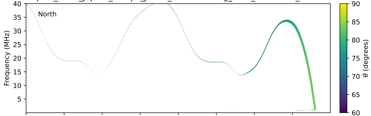
expres_earth_jupiter_europa_jrm33_lossc-wid1deg_3kev_20010105_v11.cdf
