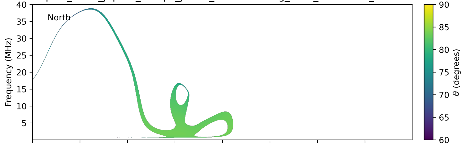
expres_earth_jupiter_europa_jrm33_lossc-wid1deg_3kev_20010102_v11.cdf
