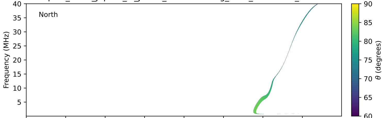
expres_earth_jupiter_io_jrm33_lossc-wid1deg_3kev_20000730_v11.cdf
