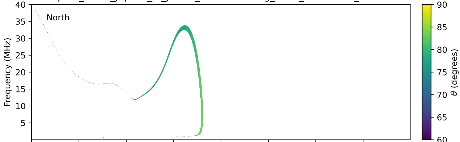
expres_earth_jupiter_io_jrm33_lossc-wid1deg_3kev_20000717_v11.cdf
