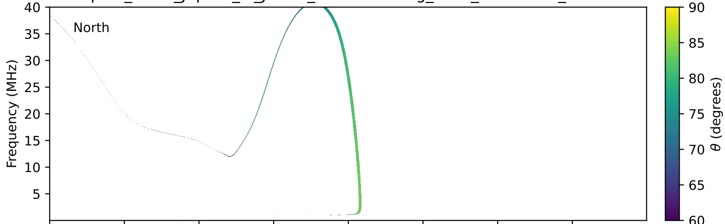
expres_earth_jupiter_io_jrm09_lossc-wid1deg_3kev_20000724_v11.cdf
