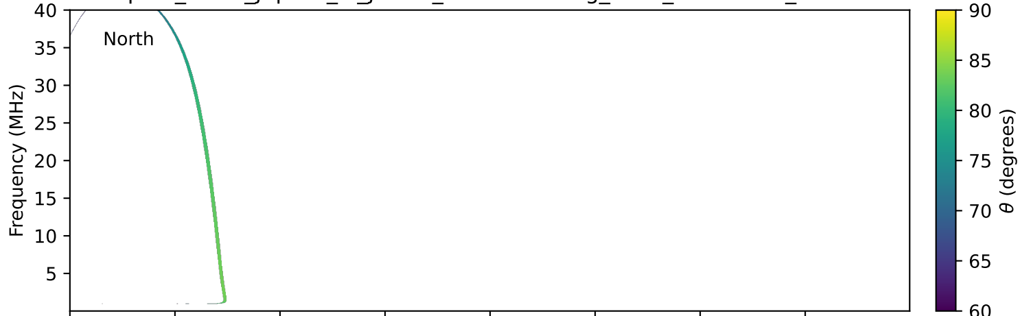
expres_earth_jupiter_io_jrm09_lossc-wid1deg_3kev_20000719_v11.cdf
