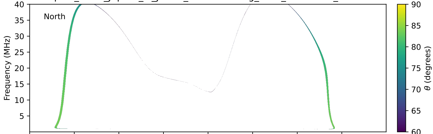
expres_earth_jupiter_io_jrm09_lossc-wid1deg_3kev_20000713_v11.cdf
