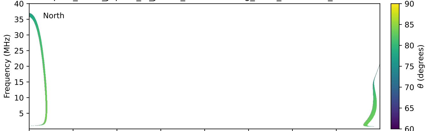
expres_earth_jupiter_io_jrm09_lossc-wid1deg_3kev_20000705_v11.cdf
