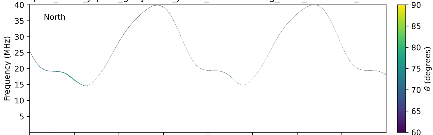
expres_earth_jupiter_ganymede_jrm33_lossc-wid1deg_3kev_20000705_v11.cdf
