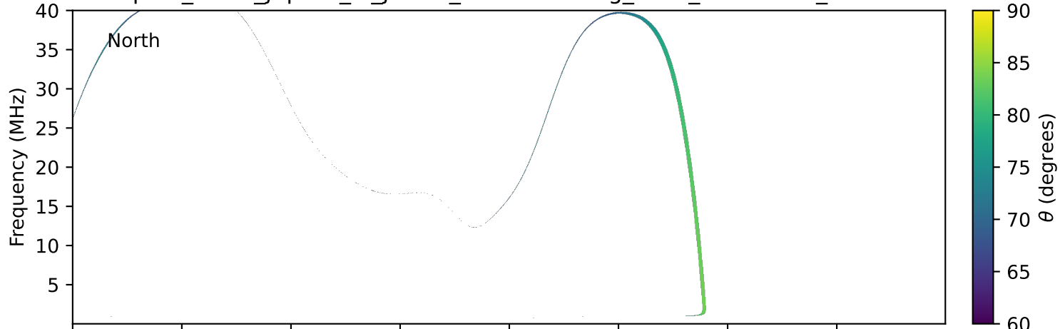
expres_earth_jupiter_io_jrm33_lossc-wid1deg_3kev_20000629_v11.cdf
