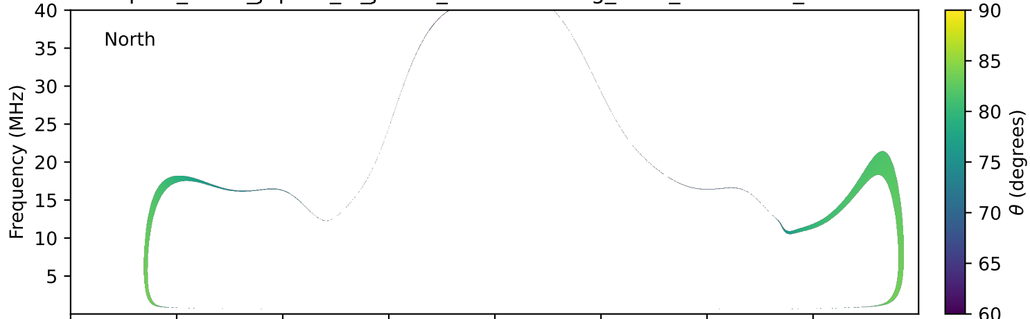
expres_earth_jupiter_io_jrm33_lossc-wid1deg_3kev_20000627_v11.cdf
