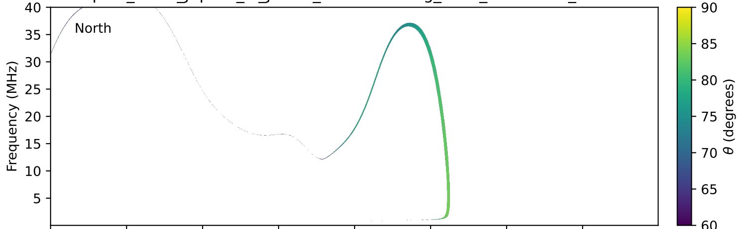
expres_earth_jupiter_io_jrm33_lossc-wid1deg_3kev_20000622_v11.cdf
