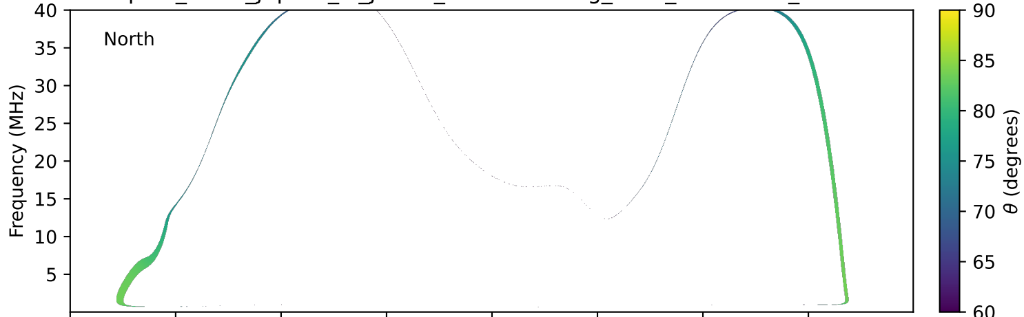
expres_earth_jupiter_io_jrm33_lossc-wid1deg_3kev_20000604_v11.cdf
