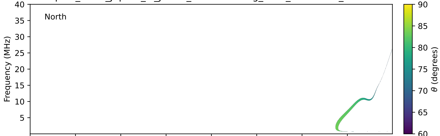
expres_earth_jupiter_io_jrm09_lossc-wid1deg_3kev_20000628_v11.cdf
