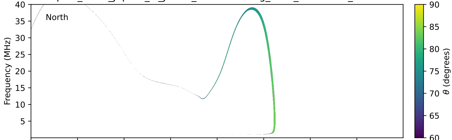
expres_earth_jupiter_io_jrm09_lossc-wid1deg_3kev_20000622_v11.cdf
