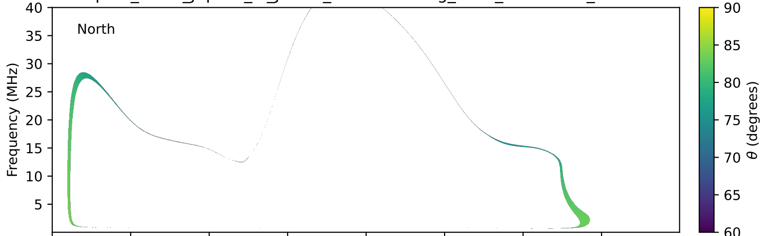
expres_earth_jupiter_io_jrm09_lossc-wid1deg_3kev_20000620_v11.cdf
