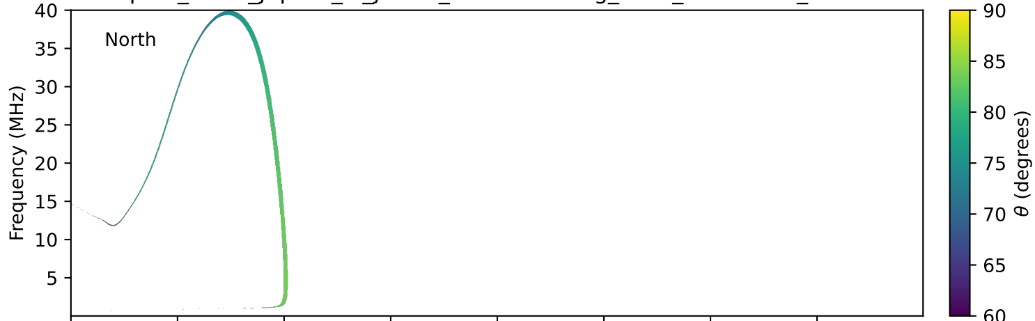
expres_earth_jupiter_io_jrm09_lossc-wid1deg_3kev_20000610_v11.cdf
