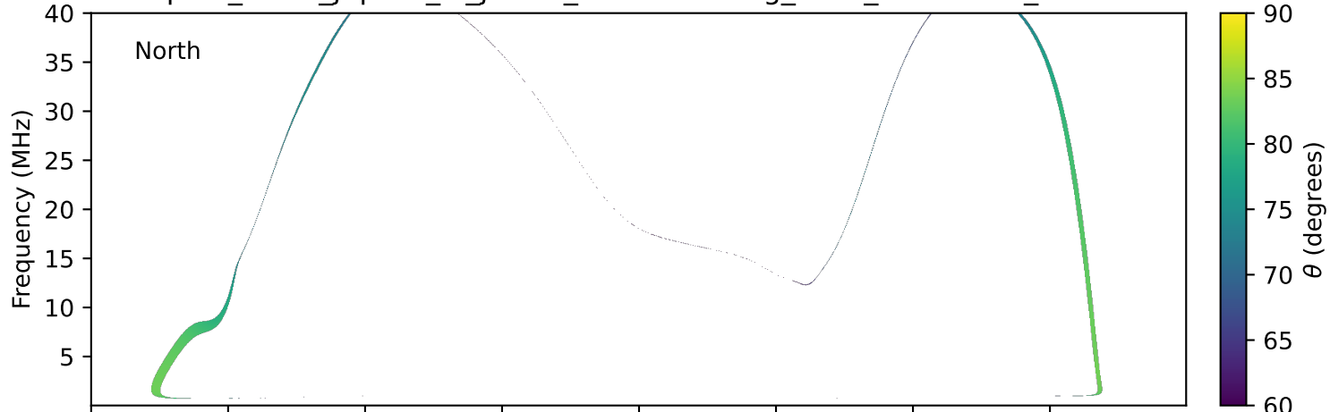
expres_earth_jupiter_io_jrm09_lossc-wid1deg_3kev_20000604_v11.cdf
