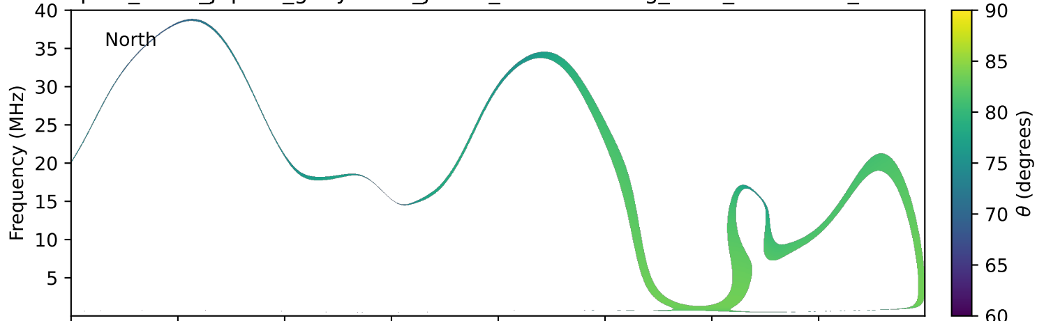
expres_earth_jupiter_ganymede_jrm33_lossc-wid1deg_3kev_20000608_v11.cdf
