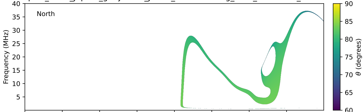
expres_earth_jupiter_ganymede_jrm09_lossc-wid1deg_3kev_20000605_v11.cdf
