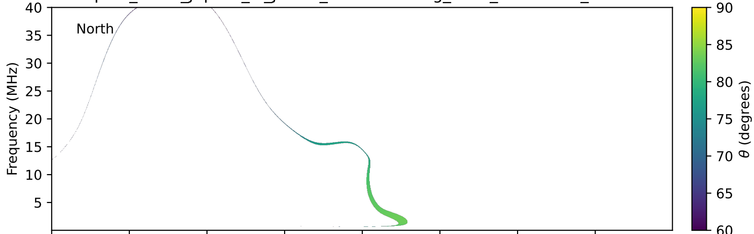
expres_earth_jupiter_io_jrm33_lossc-wid1deg_3kev_19940730_v11.cdf
