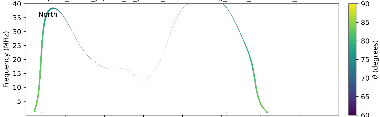
expres_earth_jupiter_io_jrm33_lossc-wid1deg_3kev_19940728_v11.cdf
