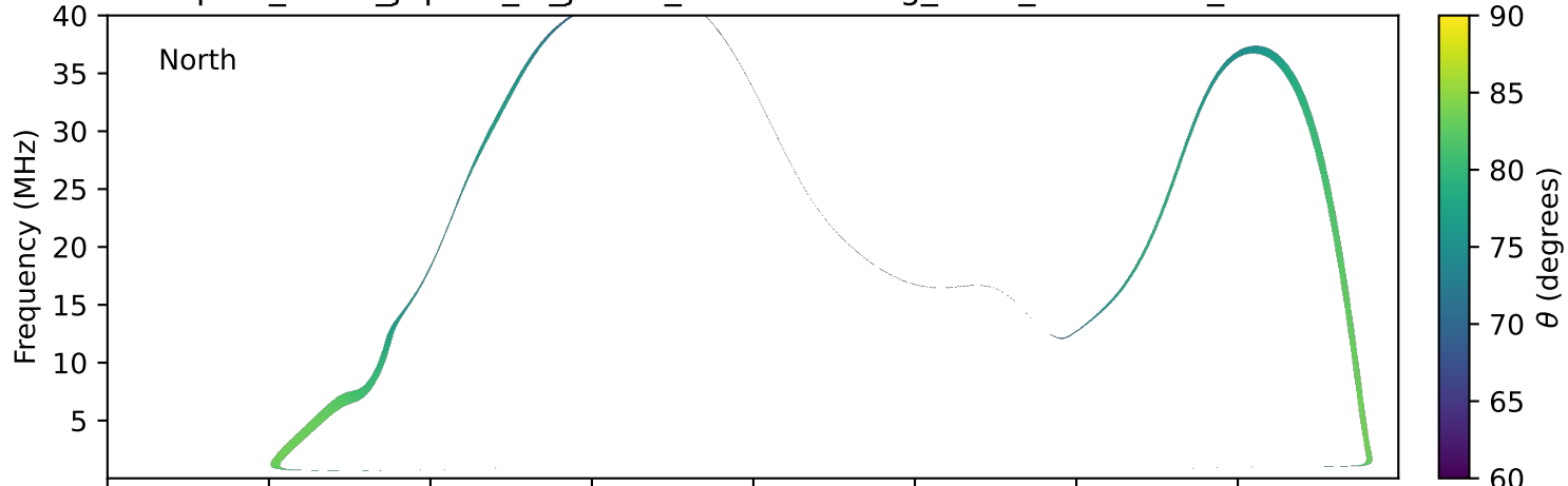
expres_earth_jupiter_io_jrm33_lossc-wid1deg_3kev_19940719_v11.cdf
