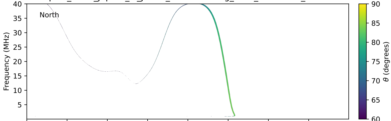
expres_earth_jupiter_io_jrm33_lossc-wid1deg_3kev_19940714_v11.cdf
