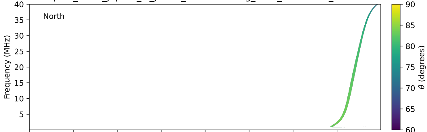
expres_earth_jupiter_io_jrm33_lossc-wid1deg_3kev_19940713_v11.cdf
