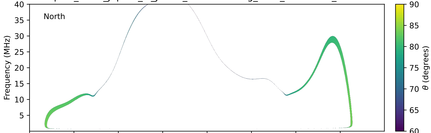
expres_earth_jupiter_io_jrm33_lossc-wid1deg_3kev_19940712_v11.cdf
