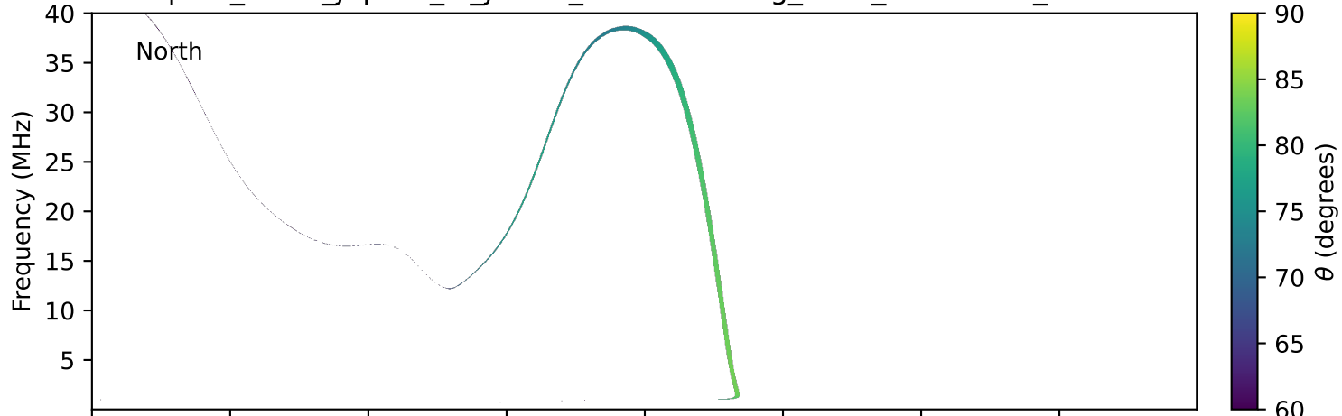
expres_earth_jupiter_io_jrm33_lossc-wid1deg_3kev_19940707_v11.cdf
