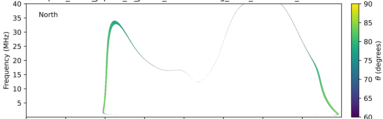
expres_earth_jupiter_io_jrm33_lossc-wid1deg_3kev_19940703_v11.cdf
