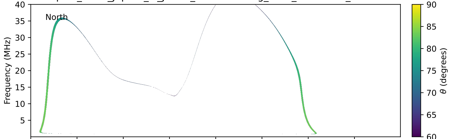
expres_earth_jupiter_io_jrm09_lossc-wid1deg_3kev_19940728_v11.cdf
