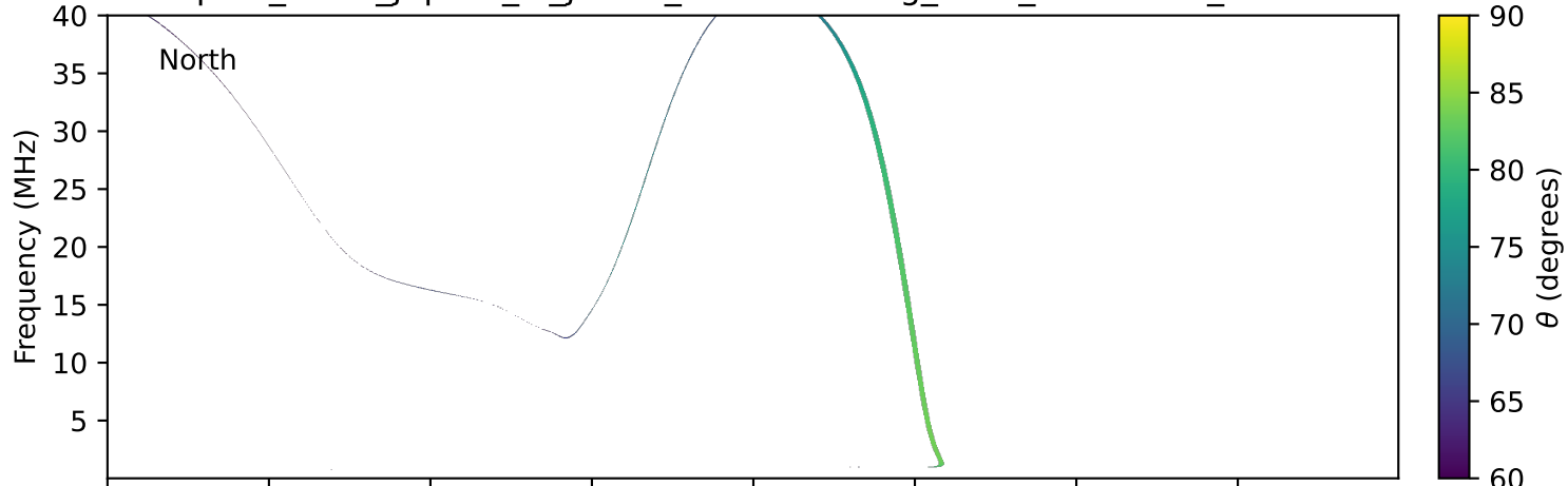
expres_earth_jupiter_io_jrm09_lossc-wid1deg_3kev_19940714_v11.cdf
