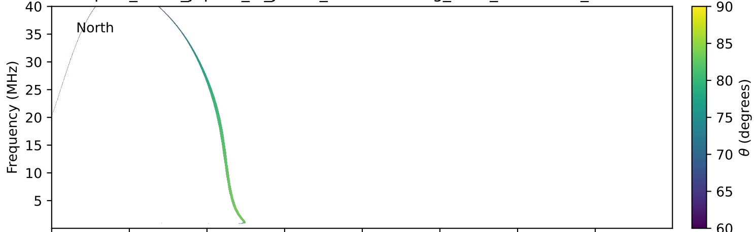
expres_earth_jupiter_io_jrm09_lossc-wid1deg_3kev_19940709_v11.cdf
