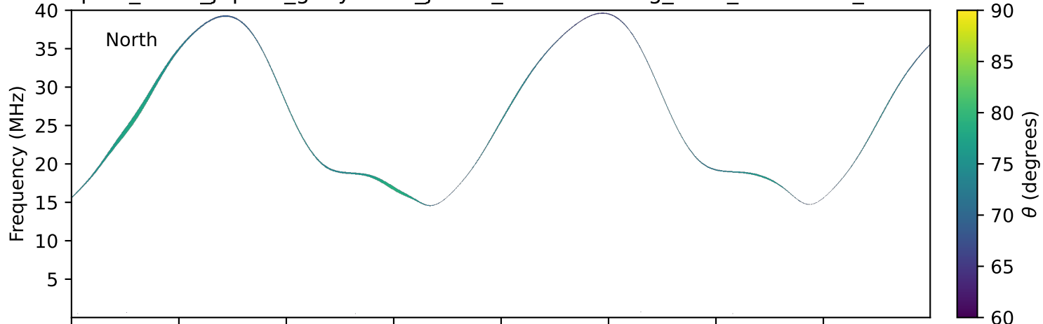
expres_earth_jupiter_ganymede_jrm33_lossc-wid1deg_3kev_19940718_v11.cdf
