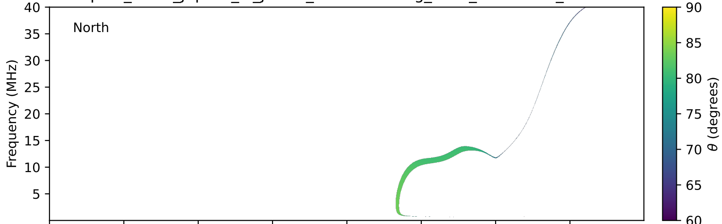
expres_earth_jupiter_io_jrm33_lossc-wid1deg_3kev_19940622_v11.cdf
