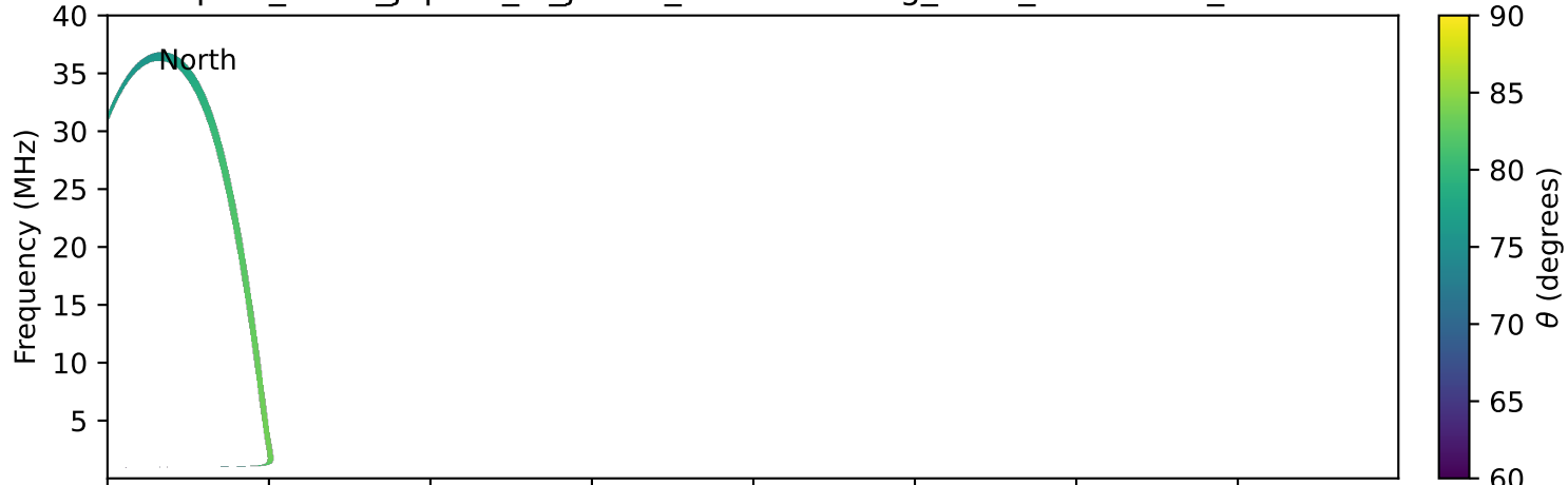
expres_earth_jupiter_io_jrm33_lossc-wid1deg_3kev_19940618_v11.cdf
