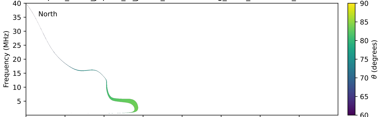
expres_earth_jupiter_io_jrm33_lossc-wid1deg_3kev_19940616_v11.cdf
