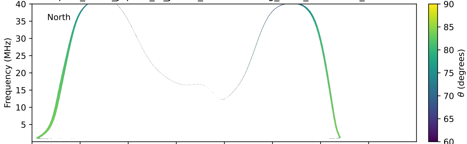
expres_earth_jupiter_io_jrm33_lossc-wid1deg_3kev_19940612_v11.cdf
