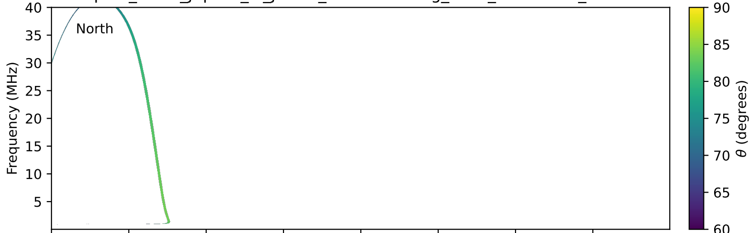
expres_earth_jupiter_io_jrm09_lossc-wid1deg_3kev_19940625_v11.cdf
