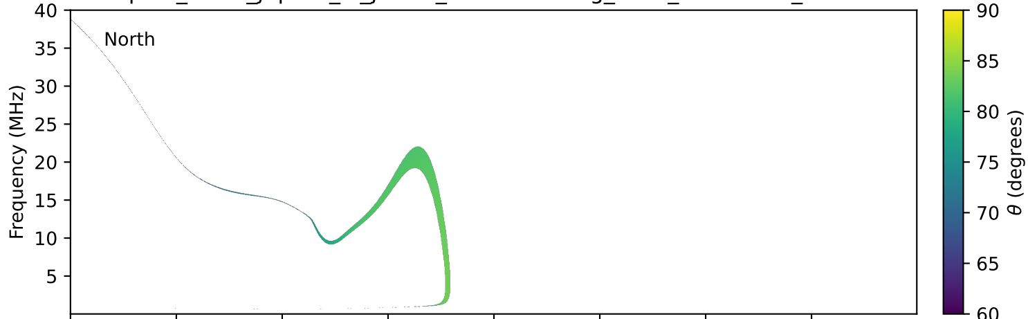
expres_earth_jupiter_io_jrm09_lossc-wid1deg_3kev_19940623_v11.cdf
