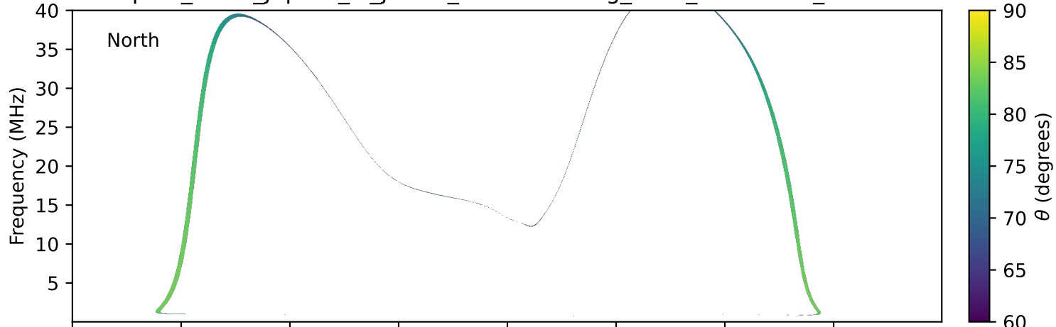
expres_earth_jupiter_io_jrm09_lossc-wid1deg_3kev_19940619_v11.cdf
